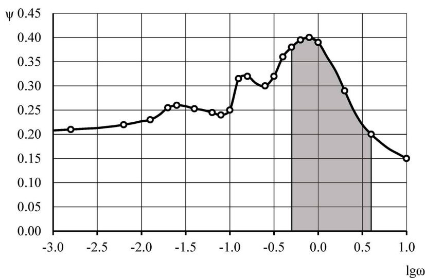
Figure 1 – Frequency dependences of the energy dissipation factor for rubber with the filling of 5.0 mass parts of carbon black
