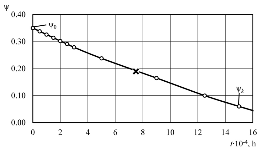
Figure 4 – Time dependence of energy absorption coefficient; \psi_0 and \psi_k are initial and final values of energy dissipation factor, x – lower limit of the vibration isolator service life
