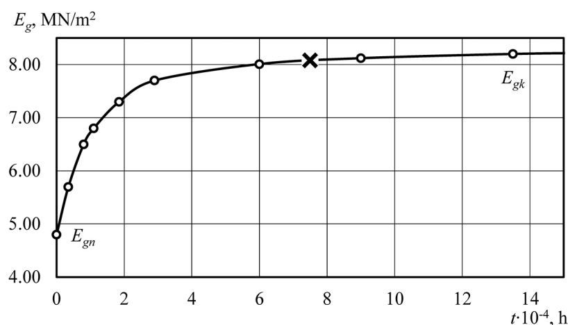
Figure 3 – Time dependence of dynamic modulus of compression; E_{gn} , E_{gk} are initial and final values of the conditionally-equilibrium modulus of elasticity, x – lower limit of the vibration isolator service life
